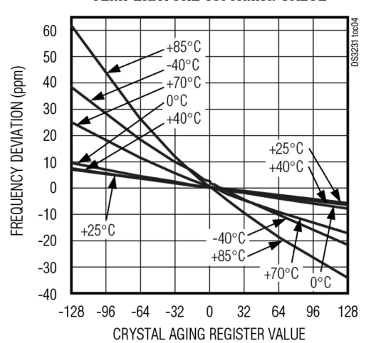
FREQUENCY DEVIATION vs. TEMPERATURE vs. AGING VALUE
